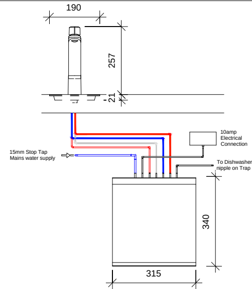
REAR VIEW
